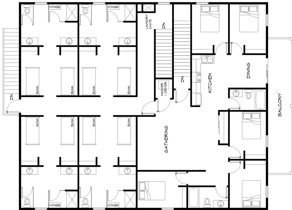
SECOND FLOOR PLAN 3000 S.F.
